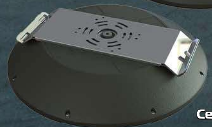
Trunnion Mount
